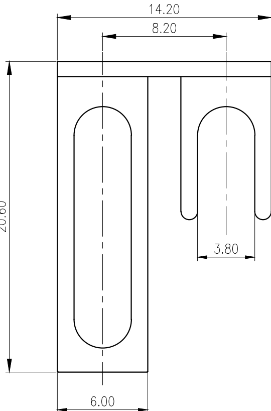
SB2 Screw
