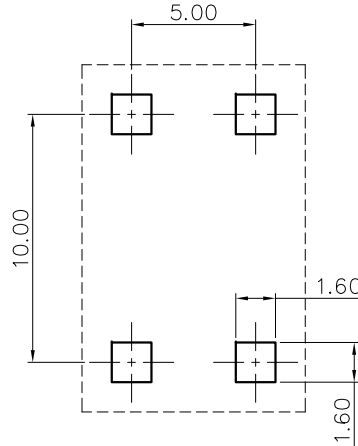
PCB LAYOUT
