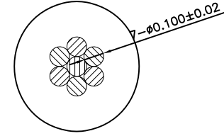
Stranded type
