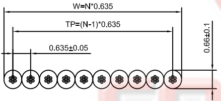
Stranded type
