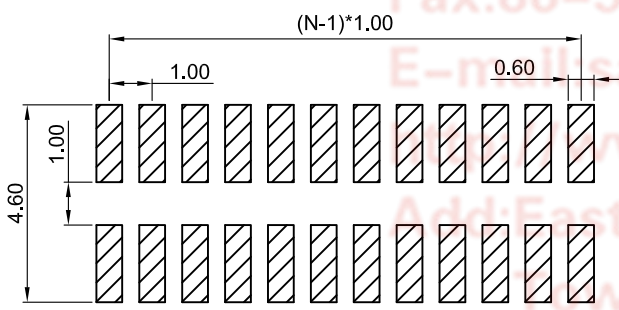
RECOMMEND PCB LAYOUT(TOLERANCE ±0.05)
