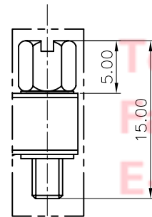
CC TYPE
