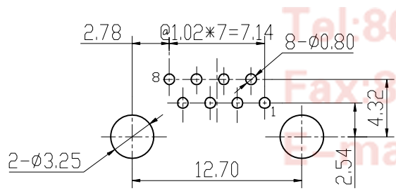
PC BOARD LAYOUT THICKNESS=1.6mm
