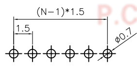
RECOMMEND PCB LAYOUT
